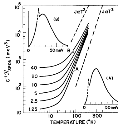
FIG. 5. Temperature dependence of the threshold current density. The parameter labeling the curves is the value of C^{-1}r_{stim}(max) , which is proportional to the gain in the active material. These values are obtained from Fig. 4, and the same conversion factors apply. The two insets show schematically the line shape and position of the lasing spike, as in Fig. 3, corresponding to the points marked A and B.
