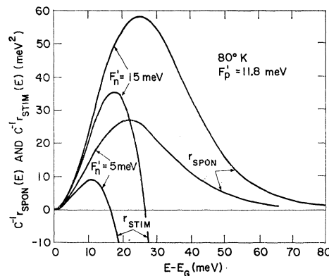
FIG. 1. Spontaneous and stimulated spectral functions at 80°K for parabolic bands, with a hole quasi-Fermi level 11.8 meV within the valence band and electron quasi-Fermi levels 5 and 15 meV within the conduction band. The spontaneous line shape is given by r_{\text{spont}} and the gain per unit length is proportional to r_{\text{stim}} . The conversion factor C is given in Eqs. (15) and (16b) for GaAs. The calculated curves shown in all the figures are based on the no-selection rule case, Eq. (6).
