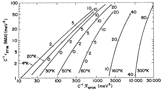
FIG. 4. Curves of C^{-1}r_{stim}(max) as functions of C^{-1}R_{spon} for a series of temperatures. The peak bulk gain, in cm^{-1} , can be obtained for GaAs by multiplying the ordinate by the factor C' in Eq. (17), and the current density can be obtained by multiplying the abscissa by the factor given in Eq. (24). The hole quasi-Fermi level is 14.6 meV at 30°K, 13.8 meV at 50°K, 1.8 meV at 160°K, and has the values given in Fig. 2 at the remaining temperatures. The electron quasi-Fermi levels, in meV, corresponding to the circled points are marked on the figure.
